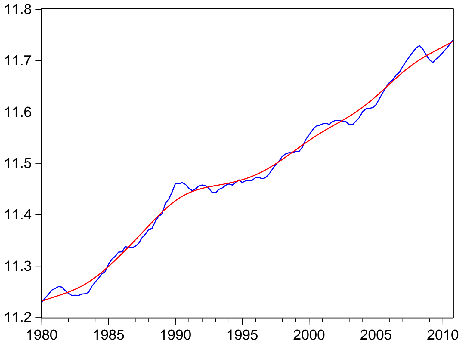
— log GDP — HP trend log GDP
